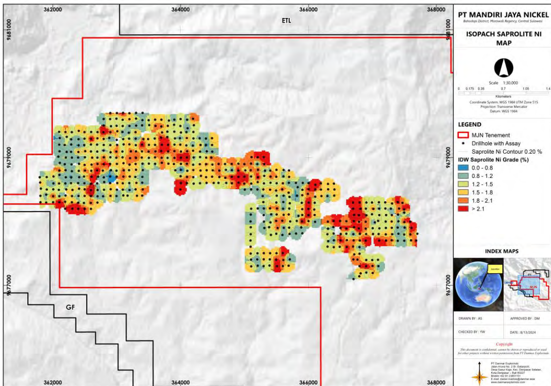
Figure 5-14 Composite nickel grade for the Saprolite zone based on drill saple assays
